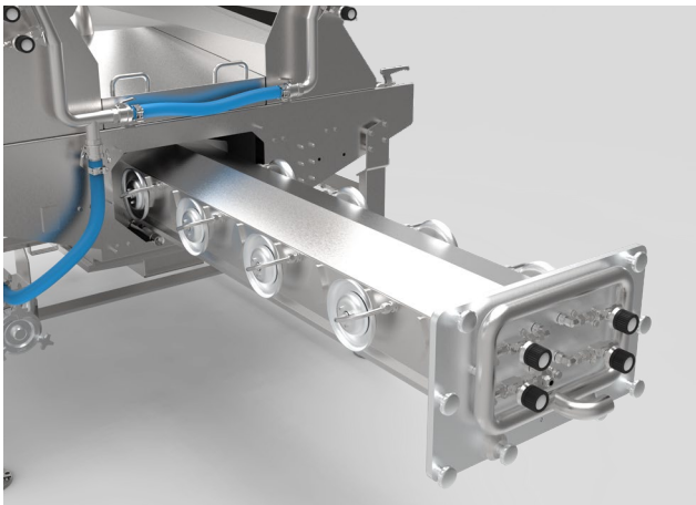
LOWER SPINNING DISC assembly removable by means of a specific trolley for easy cleaning and maintenance.
