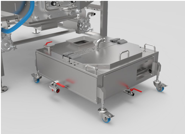
DETACHABLE JACKETED TANK of 100l with optional agitator.
