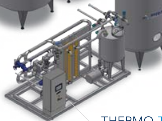
THERMO-TECH PASTEURISER
