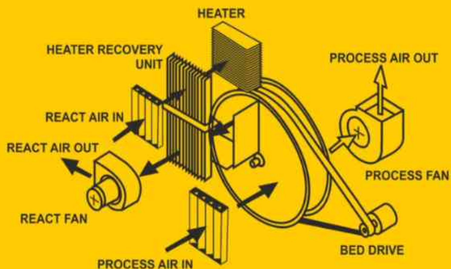
Major Components
