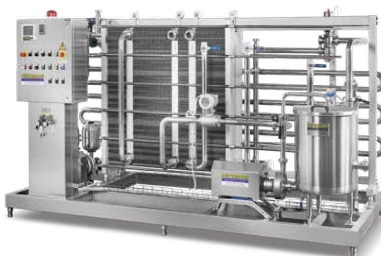
Juice and drinks thermo pasteurizer, with standard or free flow plates
